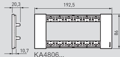
6-module cover plate
