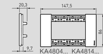
6-module cover plate
