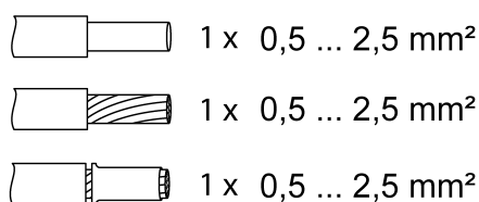
Figure 3: Clampable conductor cross-section
