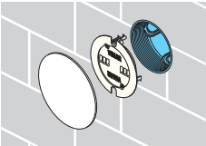
Masonry walls. The box mounting frame is fastened using claws , whereas the cover snaps into the mounting frame without leaving any screws visible.
