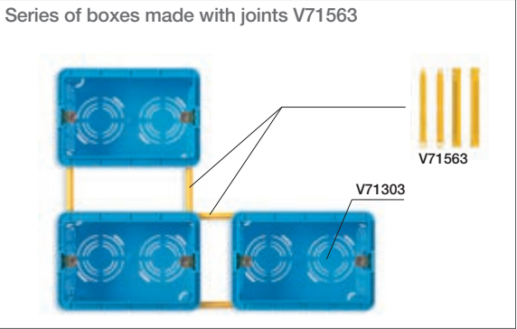
Series of boxes made with joints V71563
