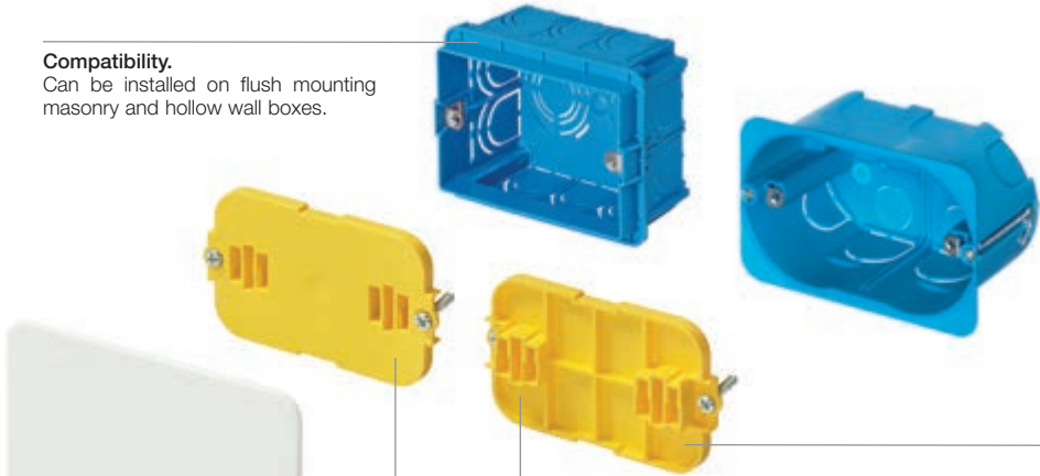
Reversible mounting frame. The mounting frame can be installed on both sides, depending on the box installation depth.
